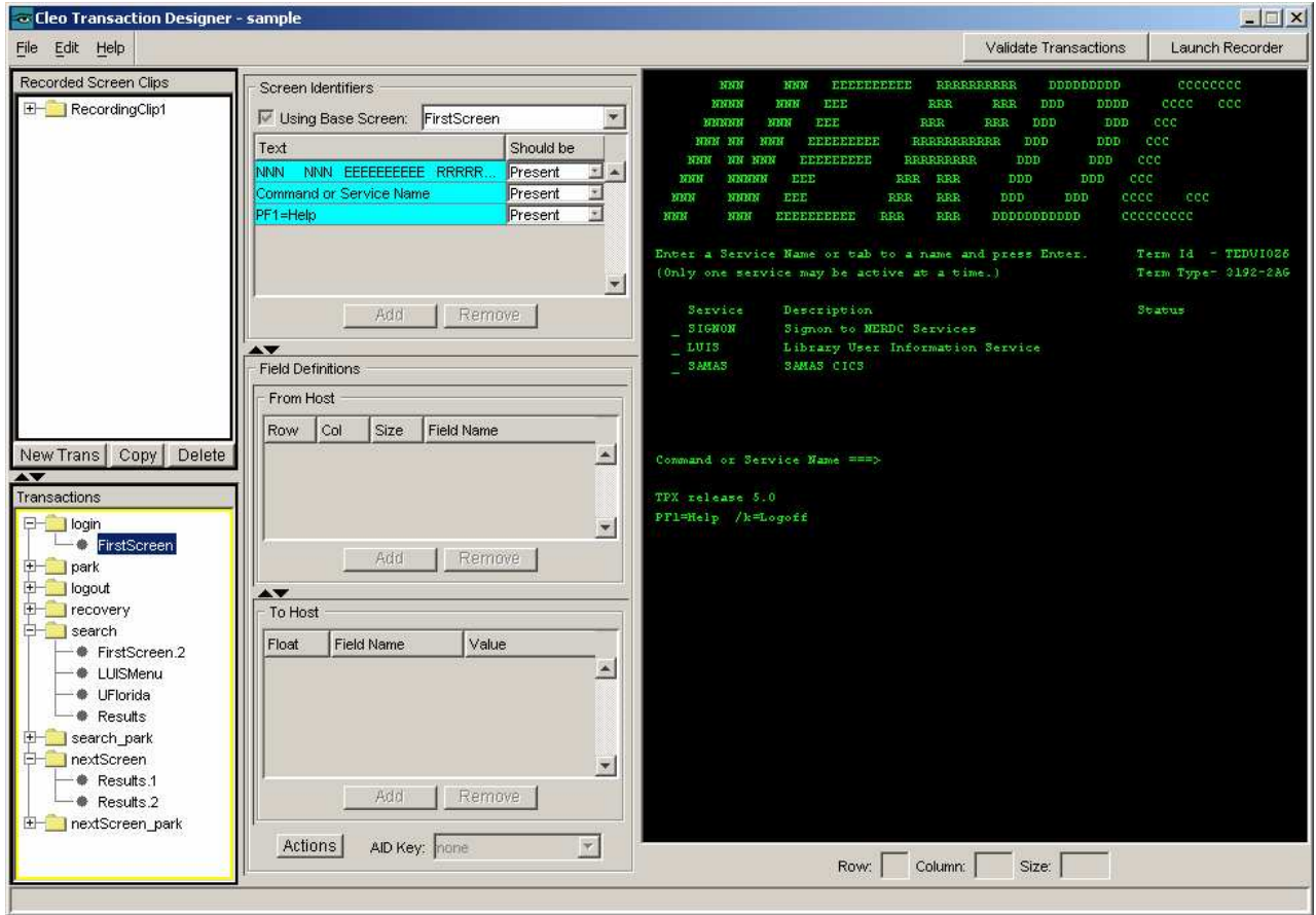
Figure 3: Transaction Set "sample"
